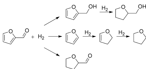
Scheme 1. Reaction pathways of furfural hydrogenation.
